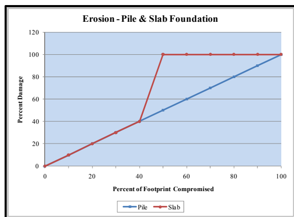
Figure 104 Pile and Slab Foundation Erosion
