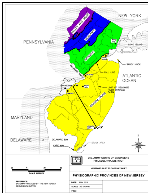
Figure 26 Physiographic Provinces.
