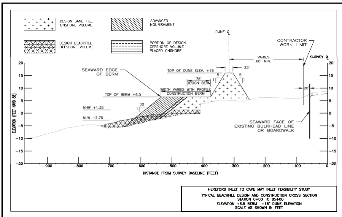
Figure 114 Wildwood and Wildwood Crest Cross Section
