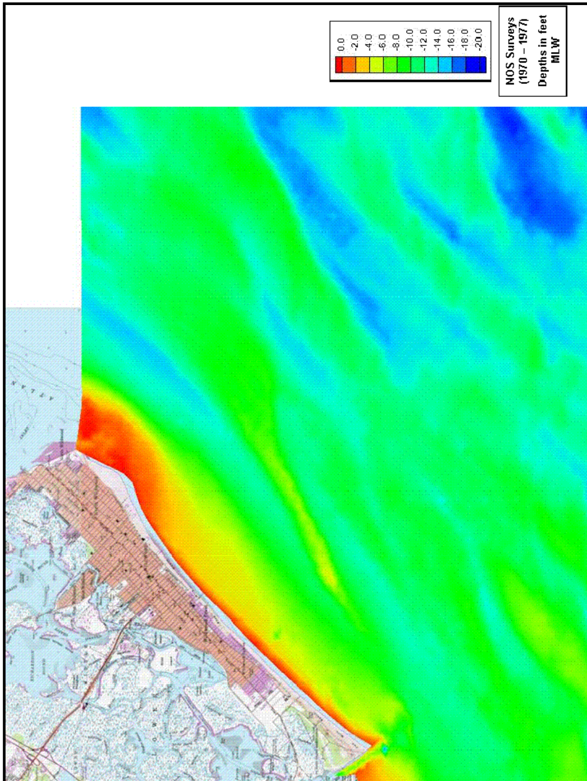
Figure 53 Wildwoods Bathymetry 1970-1977
